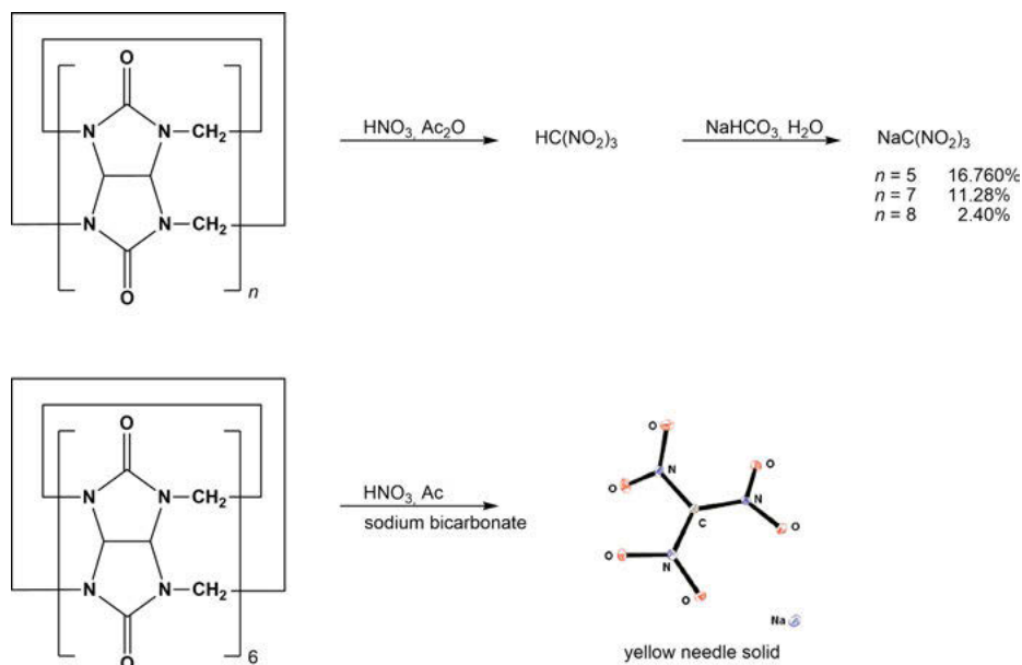
Fig. 1.23: Nitrolysis of CB.
