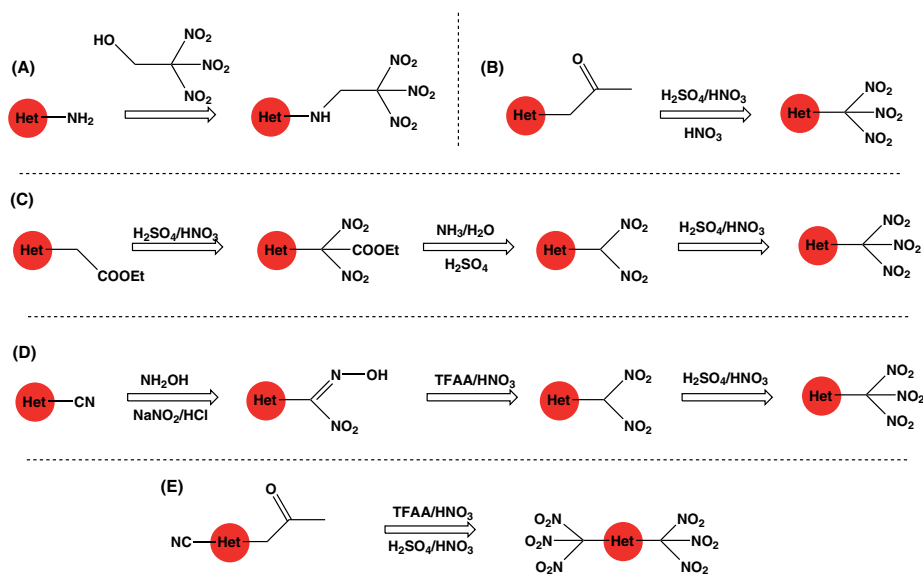
Fig. 2.13f: Synthesis of polynitro-substituted heterocyclic (Het) compounds [according to J. M. Shreeve et al., Org. Lett. 2019 , 21 , 1073 – 1077].
