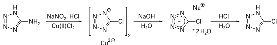
Fig. 1.18h: Synthesis of copper(II) chlorotetrazolate (CuClT).
