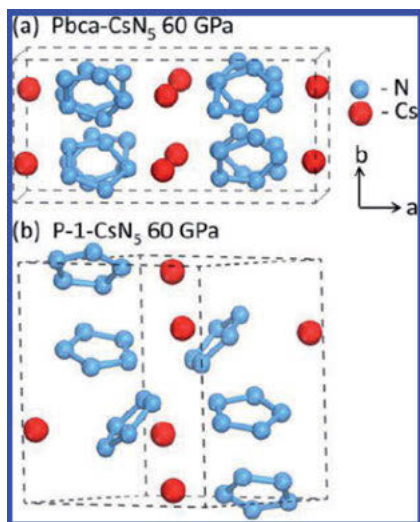
Fig. 9.5a: Crystal structures of two energetically very similar CsN 5 polymorphs at 60 GPa.
